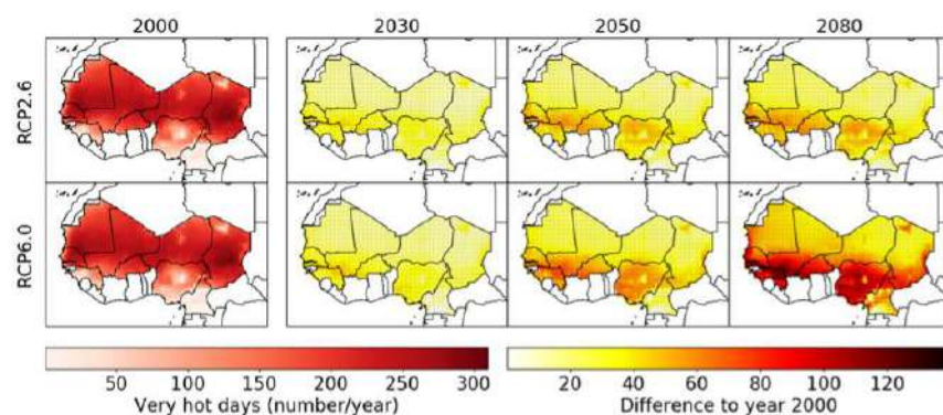
Figure 10: Projections of the annual number of very hot days (daily maximum temperature above 35°C) for the Sahel for different GHG emissions scenarios.
