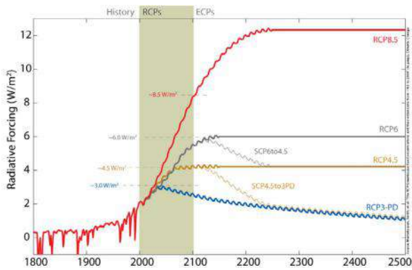
Figure 6: Global Anthropogenic Radiative Forcing for the high RCP8.5, the medium-high RCP6, the medium-low RCP4.5 and the low RCP3-PD.
