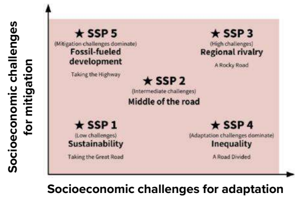
Figure 7: The SSPs of the IPCC guided scenario set (Source: O'Neill et al., 2016)
